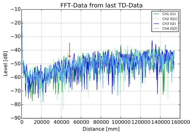
Fig. 15: Detection of the quadcopter under rainy conditions in a vertical distance of 49 m with a bandwidth of 500 MHz.
