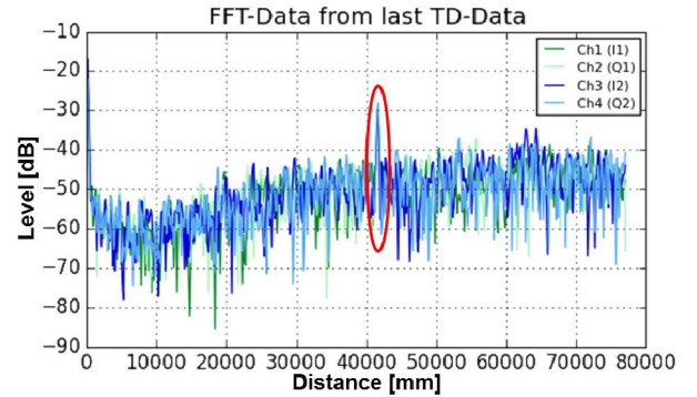
Fig. 8: Detection of the octocopter in 41.7 m vertical distance with a radar bandwidth of 1000 MHz.
