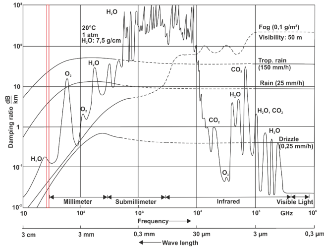
Fig. 2: Damping of electromagnetic waves through atmosphere and rain, own elaboration based on [2].
