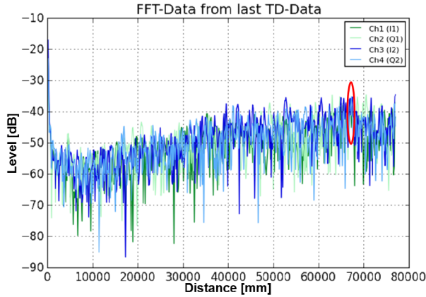
Fig. 9: Detection of the octocopter in 66.8 m height at 1000 MHz.
