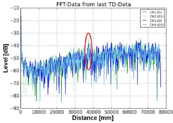
Fig. 12: Detection of the quadcopter in a vertical distance of 38 m with a bandwidth of 1000 MHz.
