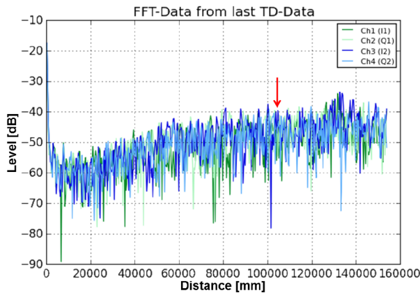
Fig. 10: Detection of the octocopter in 106.2 m distance at 500 MHz.
