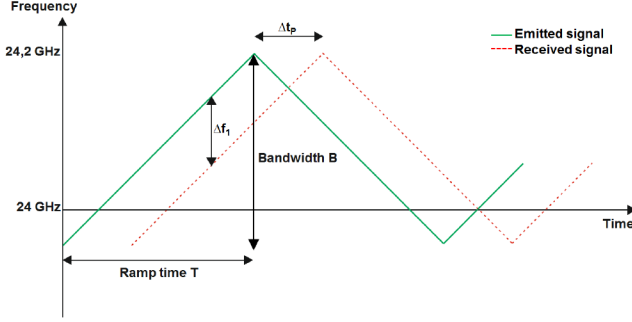
Fig. 3: Linear ramp modulation of a FMCW radar system, own elaboration.
