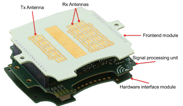
Fig. 1: Sandwich structure of the IMST 24 GHz radar system, own elaboration based on [4].
