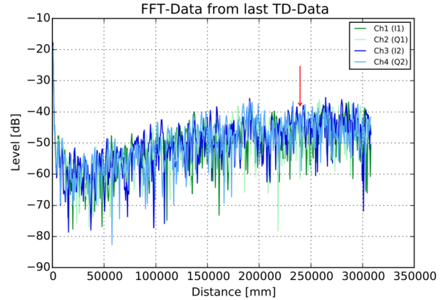
Fig. 11: Detection of the octocopter in 237.7 m distance with a radar bandwidth of 250 MHz.
