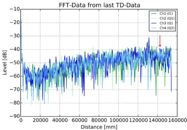
Fig. 13: Detection of the quadcopter in a distance of 143 m with a bandwidth of 500 MHz.
