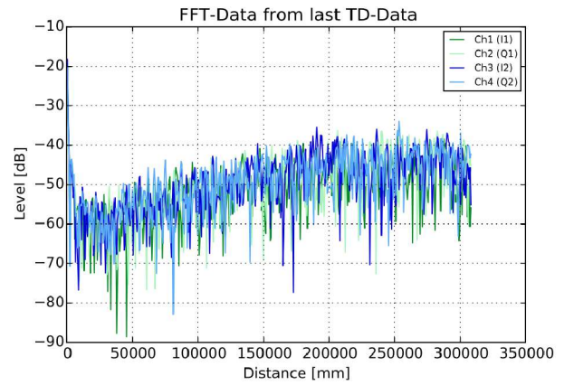
Fig. 14: Background identification of the test airspace under rainy conditions with a bandwidth of 250 MHz.
