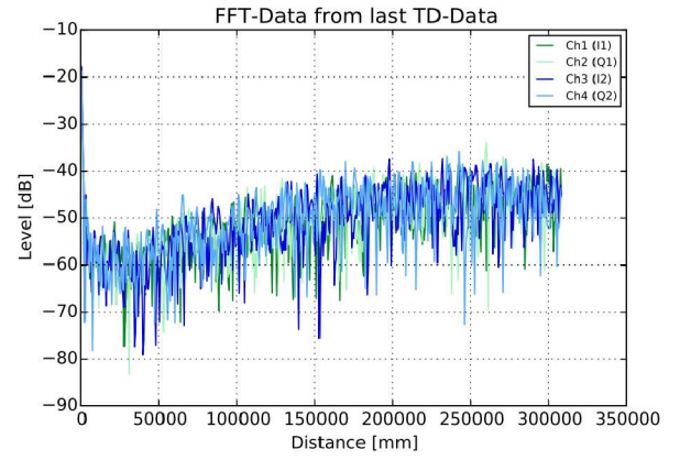
Fig. 7: Background identification of the test airspace with a radar bandwidth of 250 MHz.
